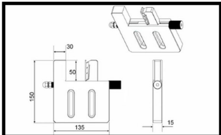
Set morsa Inox SU-MR-1550
